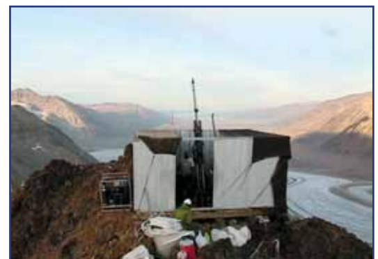
Heli-portable equipment
