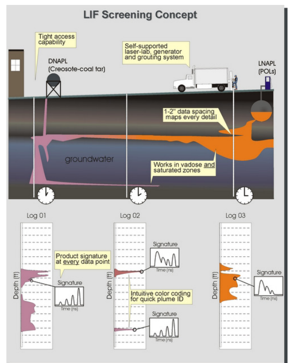
Figure Concept: Laser induced fluorescence offers a fast and efficient means for delineating PAH contaminant plumes. (Figure courtesy of Dakota Technologies)
